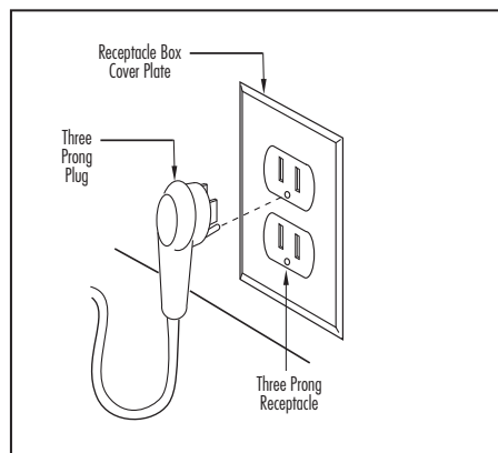
Fig. 15a Connecting the range to the power supply - RGU &amp; RGUC Models
