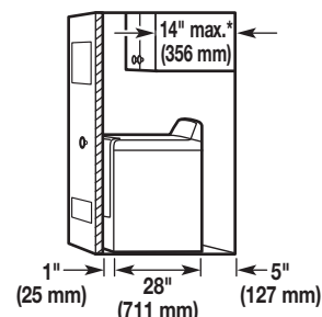
Side view - closet or confined area (Dryer with flat back)
