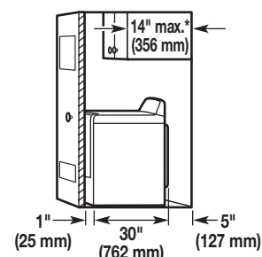
Side view - closet or confined area (Dryer with extended back)
