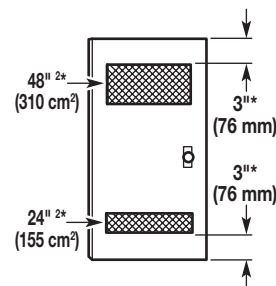
Closet door with vents
