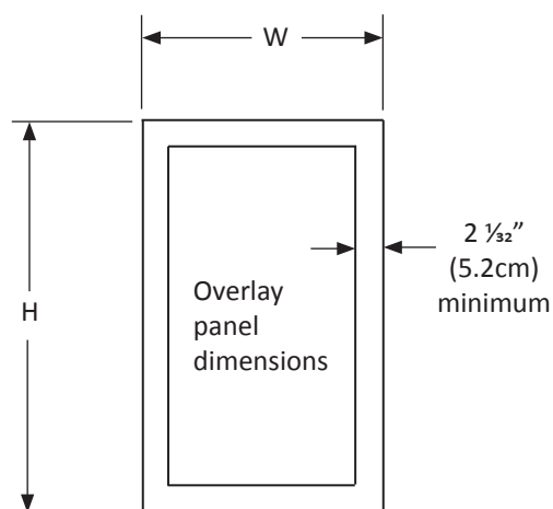
Figure 8 Glass Door Models and Solid Door Models
