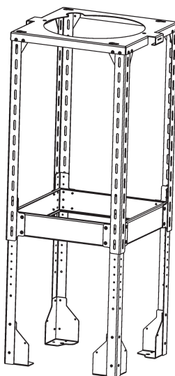
SUPPORT FRAME
