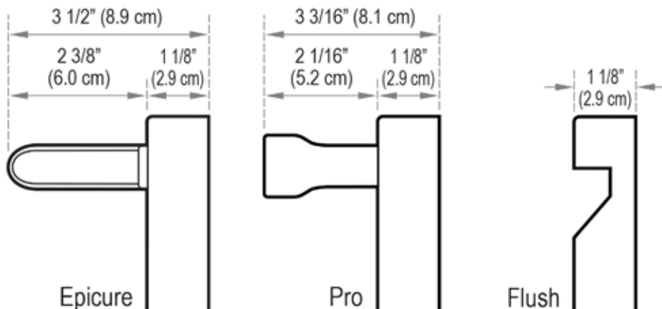
Handle Profile Dimensions
