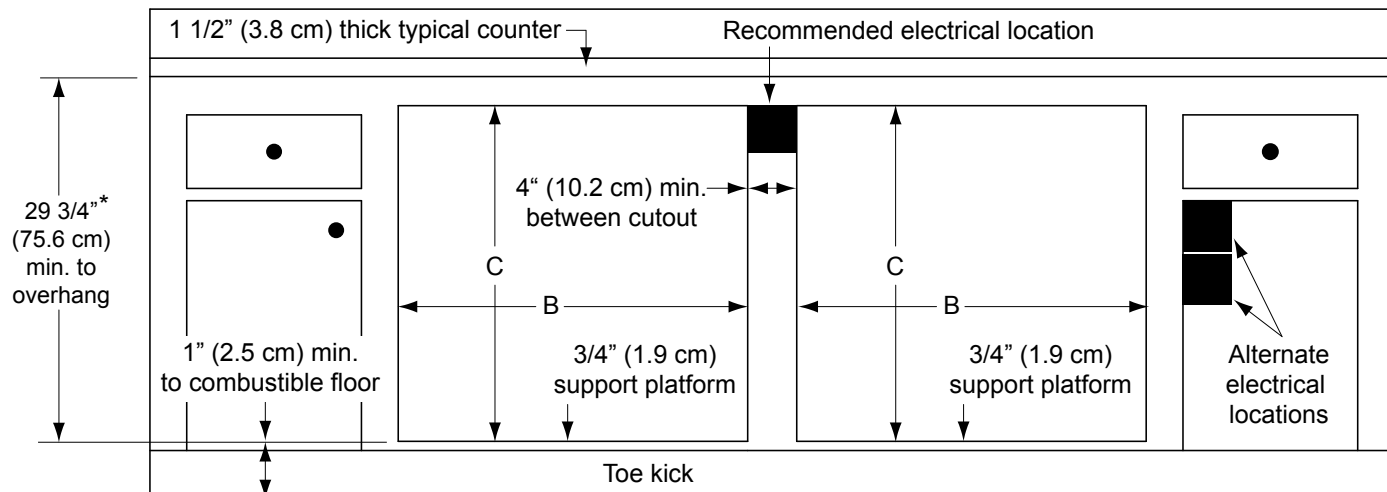
Two Single Wall Ovens - Installed Under Counter
