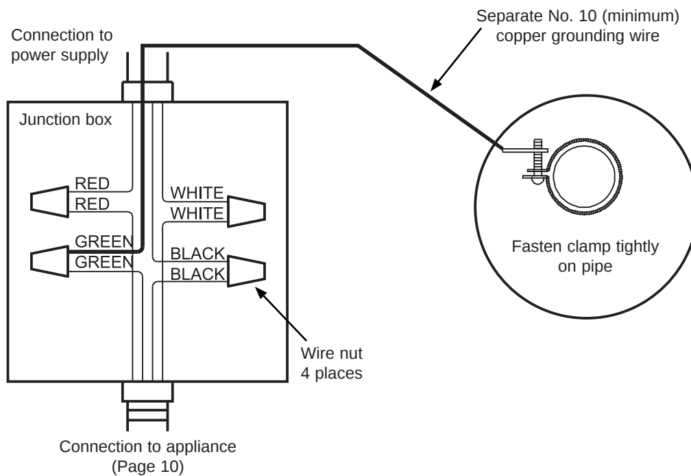
4 Wire Conduit Connection to Junction Box with External Ground
