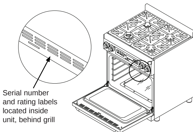
Model and Serial Number Location
