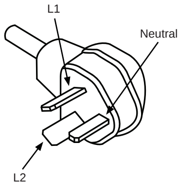
3-Wire Appliance Cord Plug
