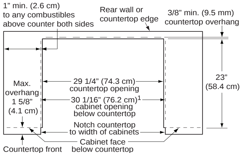
Top View - Slide-In, Self-Rimming Installation, 3" Side Panels Removed - Min. Required Cabinet Depth: 23 3/8"
