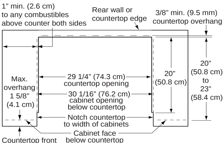
Top View - Slide-In, Self-Rimming Installation, 3" Side Panels Installed - Cabinet Depths 20 3/8" to 23 3/8"
