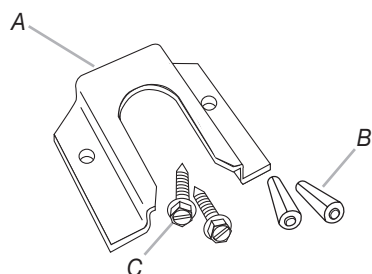
A. Anti-tip bracket B. Plastic anchors (2) C. #10 x 1" (2.5 cm) screws (2)
