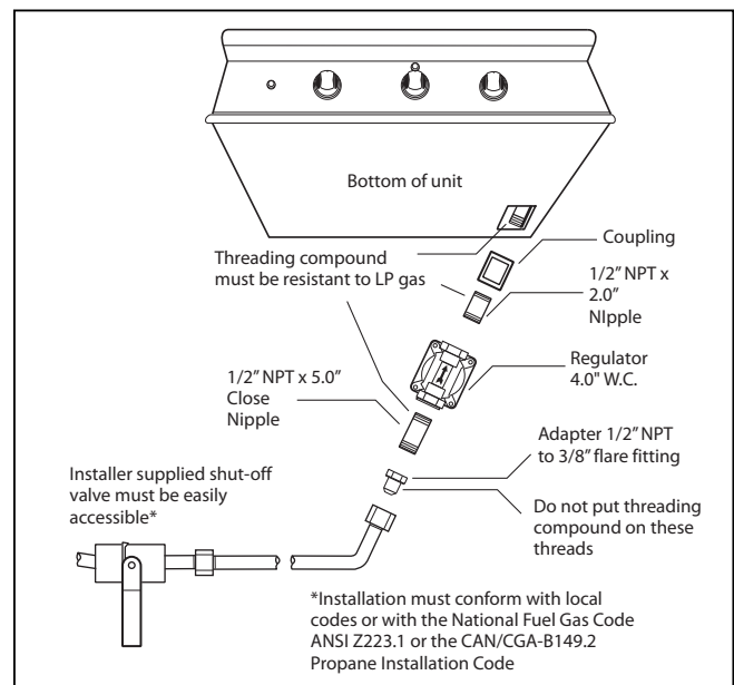
FIG. 22 Natural Gas
