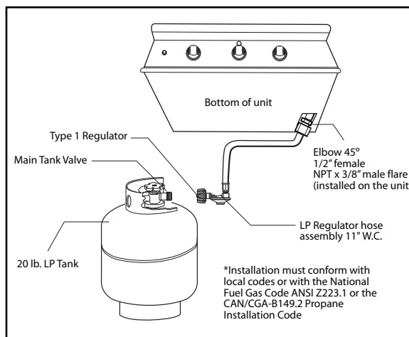
FIG. 23 LP Gas
