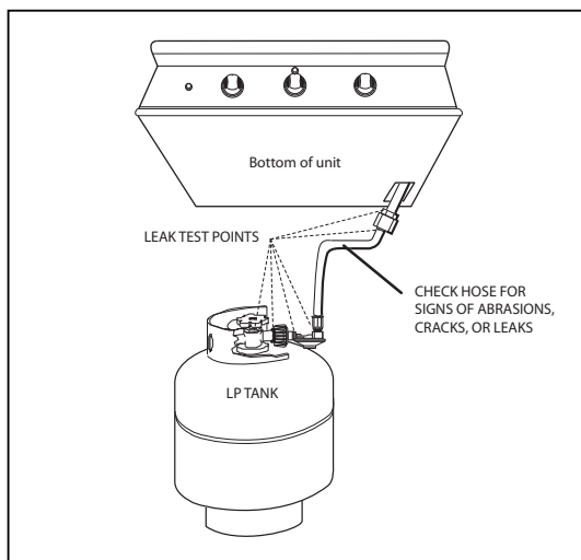
FIG. 30 LP Gas
