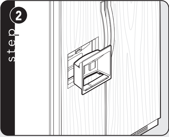
Locate opening in door and position bezel. Note: Graphics on bezel will be on top end, tilt slightly forward to allow water tube clearance.
