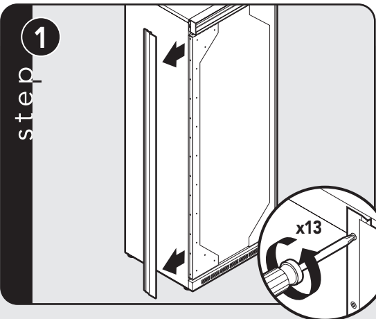
Remove handle side cabinet screws and trim with a phillips screwdriver.
