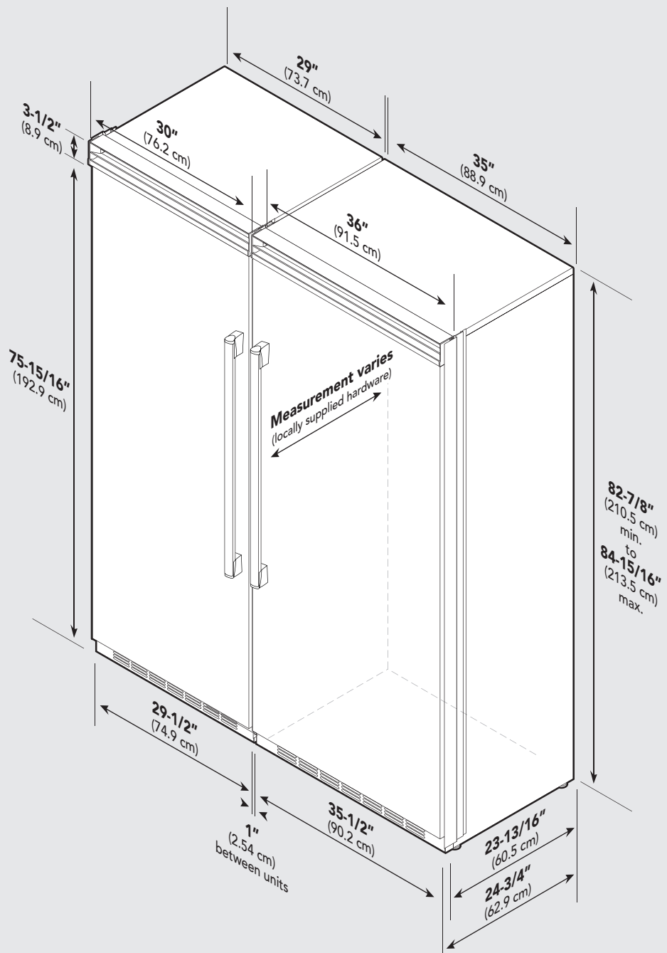
Dual 30" & 36" All Refrigerator/Freezer
