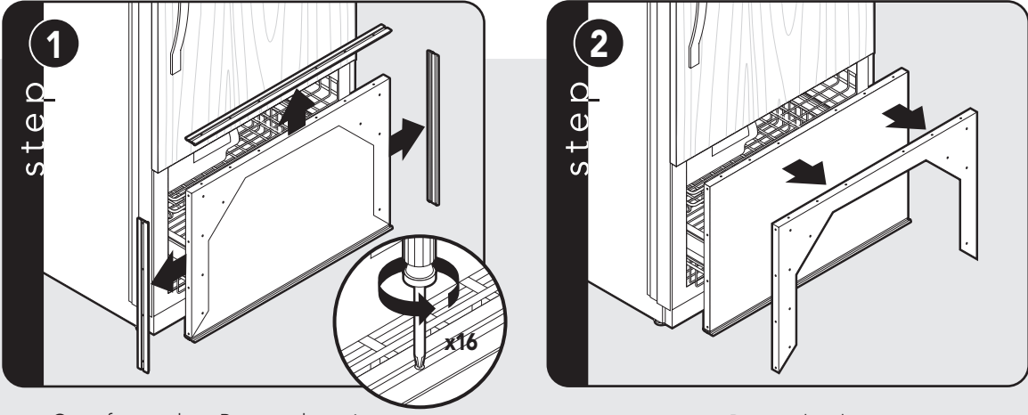
Open freezer door. Remove door trim screws and door trim with a phillips screwdriver.
