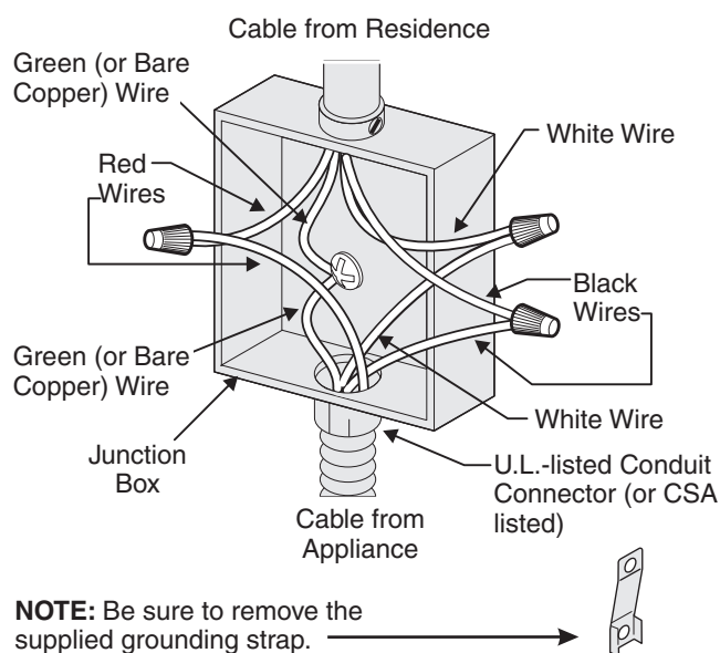
Figure 11 – 4-Wire Electrical System (Example: Junction Box)
