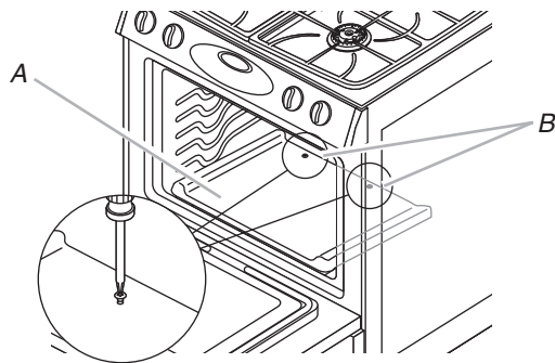
A. Oven bake burner cover B. Oven bake burner cover screws
