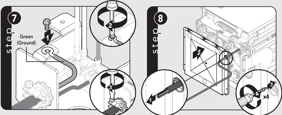
Connect ground wire. Tighten screws on strain relief. Note: Reinstall terminal block cover and front plate. Run wire through grommet on bottom pan. Replace bottom pan.
