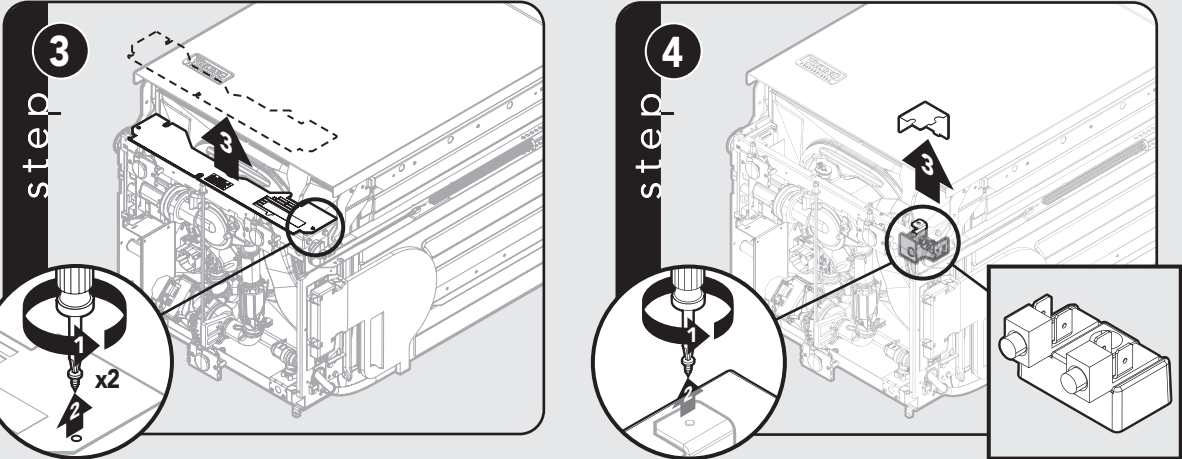
Remove front plate. Remove terminal block cover. Remove factory installed power cable from terminal block.
