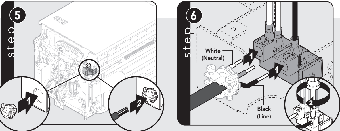
Attach UL approved 3/4" strain relief (not included) to bottom of terminal box. Run wires through strain relief. Connect wires to terminal block.
