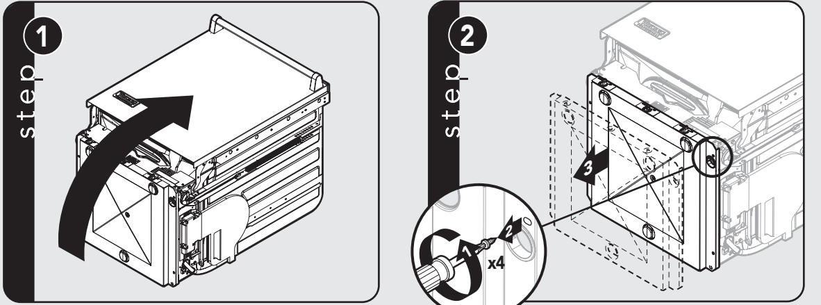
Remove any loose items in the dishwasher and carefully lay the dishwasher on its back. Note: Be careful not to pinch hoses or power cord beneath dishwasher. Remove bottom pan. Note: Rapid removal of the bottom pan will cause damage to the moisture sensor. For installation and servicing, slowly pull the bottom pan from the unit and disconnect the wire from the moisture sensor, which is located in the center of the pan.
