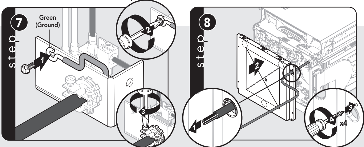
Connect ground wire. Tighten screws on strain relief. Note: Reinstall front plate. Run wire through grommet on bottom pan. Replace bottom pan.
