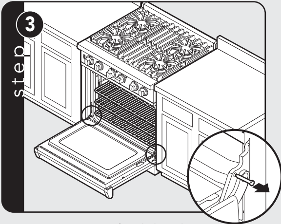
Remove pins from holes in hinges.
