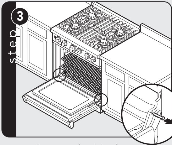
Remove pins from hole in hinges.
