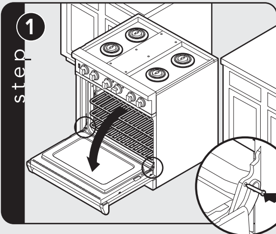
Open door completely. Place pins, supplied with unit, in pin hole. For personal safety, ONLY use pins supplied with the unit.
