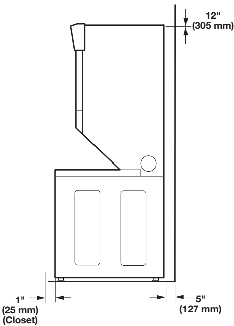
Front/Back/Top Clearances
