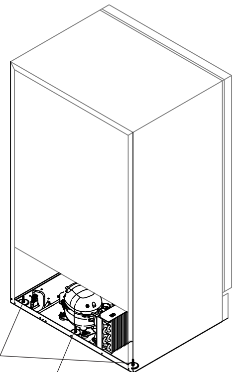
Figure 3 Rear of unit with access cover removed
