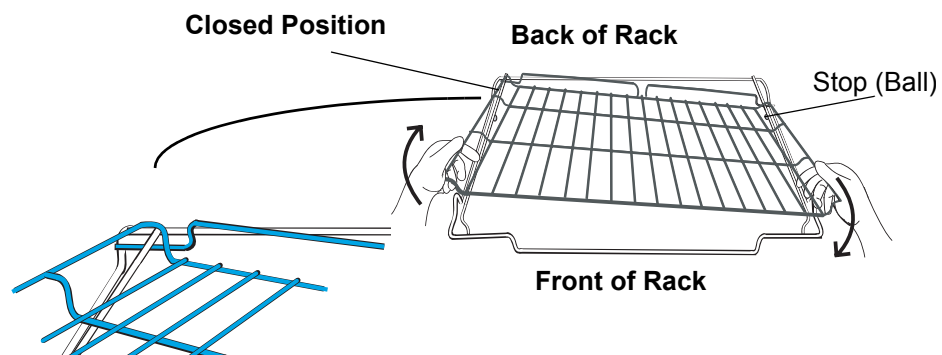
Figure 5: Disassembly
