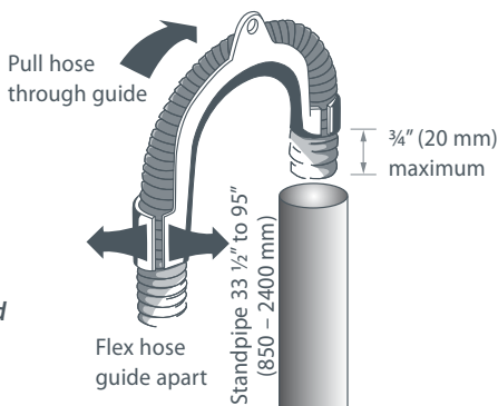
Fig.4 Fitting the drain hose guide
