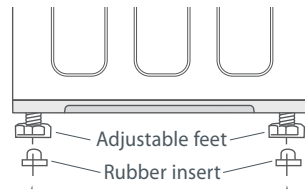
Fig.7 Leveling – Step 1 & 2
