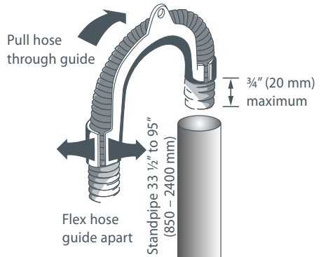
Fig.3 Fitting the drain hose guide
