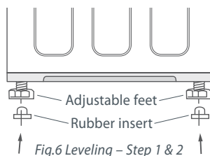
Fig.6 Leveling – Step 1 & 2
