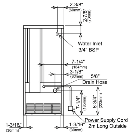
Back Dimensions
