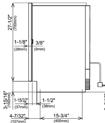
Side Dimensions
