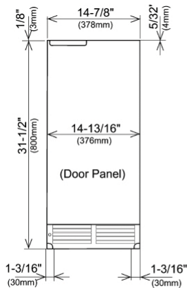
Front Dimensions
