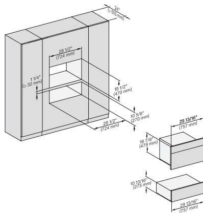
H6x70BM, ESW6x80, DGC7x7x(X), H7x70BM(X), ESW7x80, DGC676x, NA7000 Fitting Combi wide front, Installation drawing, Proud, NA
