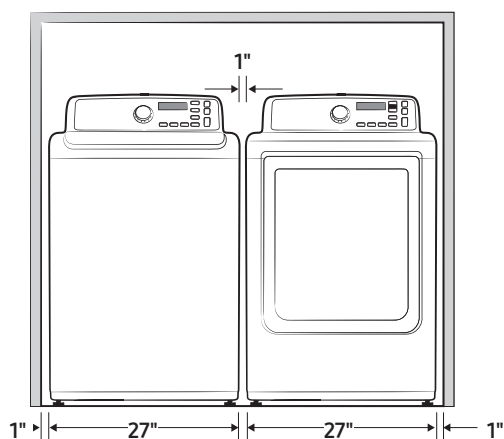
Recessed Area
