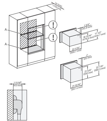
H 6560B, EBA 6808, H 6x60BP, H 6x70BM, H 7xxxBM/BMX, EBA 7868 Installation Combi, Installation drawing, Flush inset, NA
