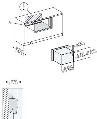
H 6x70 BM, H7x70BM(X) installation of built-under with wide front, installation drawing, Flush inset, NA
