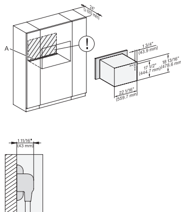
H 6x70 BM, H7x70BM(X), installation, installation drawing, Proud, NA
