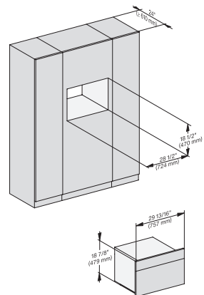
H 6x70 BM, H7x70BM, DGC7x7(X), fitting, installation drawing, Proud, NA
