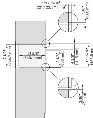
(DG 6x00 + H 6x00 BM) + EBA 6808, H7x4x40 BM (+EBA7848) side view, installation drawing, Proud, NA
