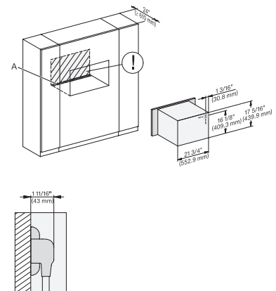
H 6x00 BM + EBA 6808, H7x40 BM (+EBA7848) wide front installation, installation drawing, Proud, NA
