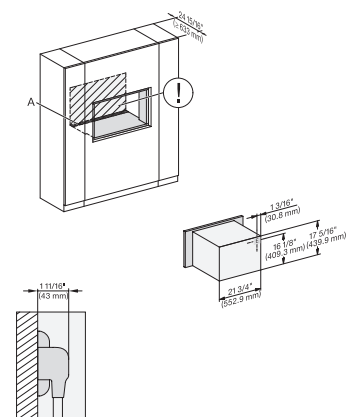
H 6x00 BM + EBA 6808, H7x40BM(+EBA7848), wide front installation, installation drawing, Flush inset, NA
