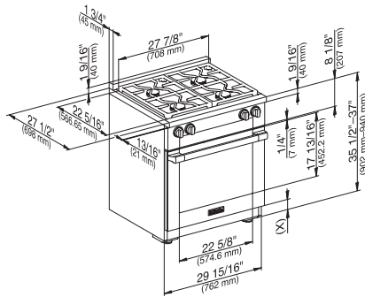
HR1924 (installation drawing)
