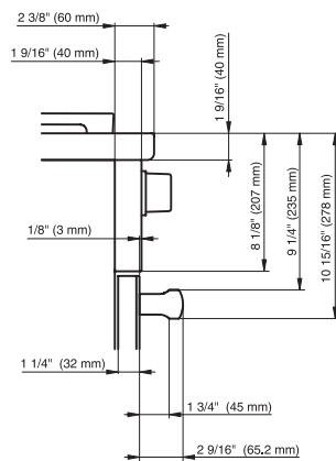
HR19x4, HR193x, HR195x (installation drawing)
