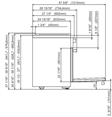
HR1924 (installation drawing)
