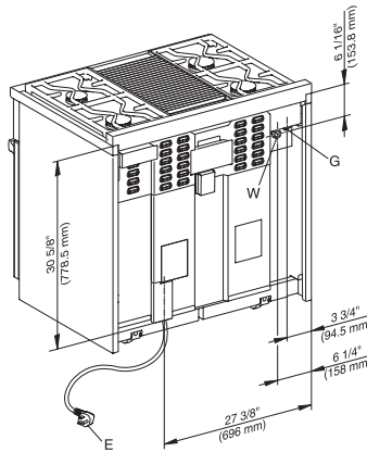
HR1935G (installation drawing)
