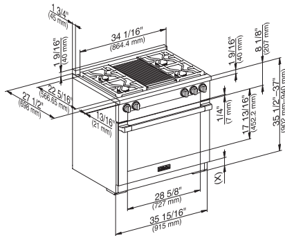
HR1935G (installation drawing)
