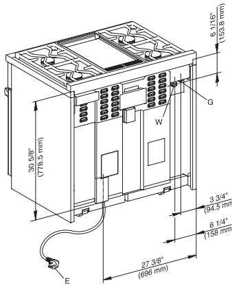
HR1936G (installation drawing)
