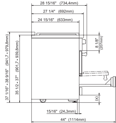
HR19xx (installation drawing)
