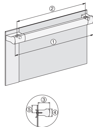
H195x installation drawings
