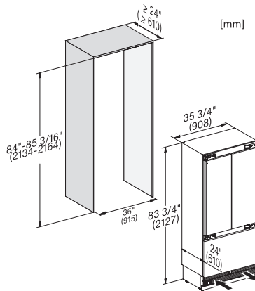
KF2982Vi, KF2981Vi, installation, MasterCool, installation drawings
