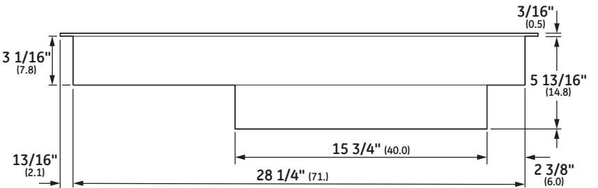
FRONT VIEW
