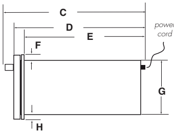
WDU-30 DIMENSIONS Side View
