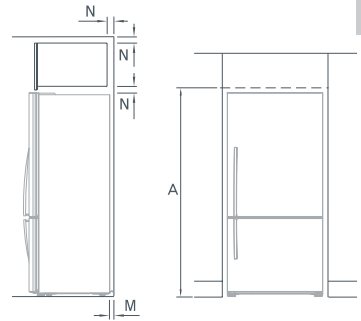
Flush with refrigerator door – 90° door rotation
