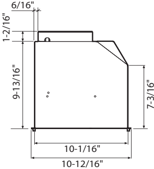
› Side of hood
