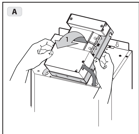
Fig.3A: Lift the electrical plant box.
