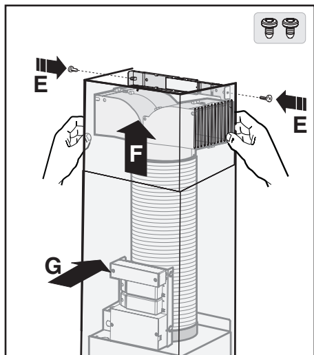
Fig.7: Place the bottom flue G on top of the frame. Then pull out the top flue F to the bracket and fasten it using the 2 screws E .
