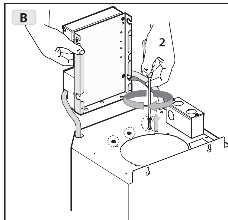
Fig.3B: Remove the 3 fixed screws.
