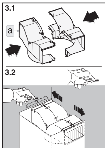
Fig.3: Put together the two parts of the air deviator as shown in picture no 3.1. It may be necessary to cut the deviator to fit the width of the chimney as shown in picture 3.2 A sharp blade or Hacksaw is recommended to trim the plastic.
