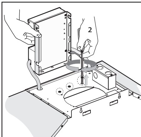
Fig.3B: Remove the 3 fixed screws.
